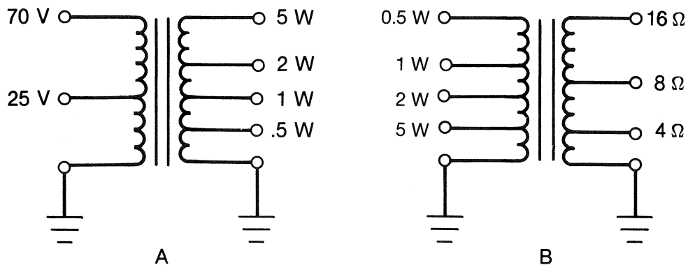
FIGURE 2. TYPICAL 70-VOLT DISTRIBUTION TRANSFORMERS
