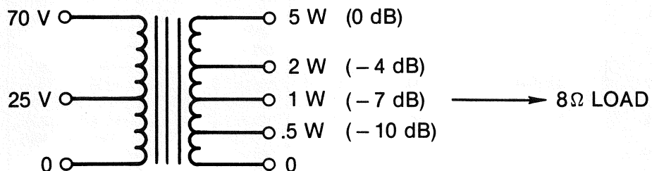
FIGURE 4. JBL MODEL 9315HT TRANSFORMER
