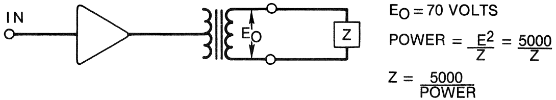
FIGURE 1. A 70-VOLT AMPLIFIER
